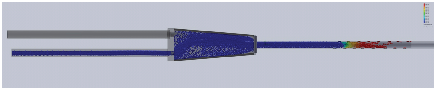
FIGURE 3. Internal flow velocity distribution according to pressure change within the catheter lumens. Computational fluid dynamics visualization of the internal hemodynamic profile. The color gradient indicates variations in flow velocity, with a recorded maximum of 12.69 m/s localized at the narrowest cross-sections of the catheter. These high-velocity regions correspond to transient peaks in shear stress (maximum 2,602.45 Pa), characterized by extremely brief erythrocyte transit times.
