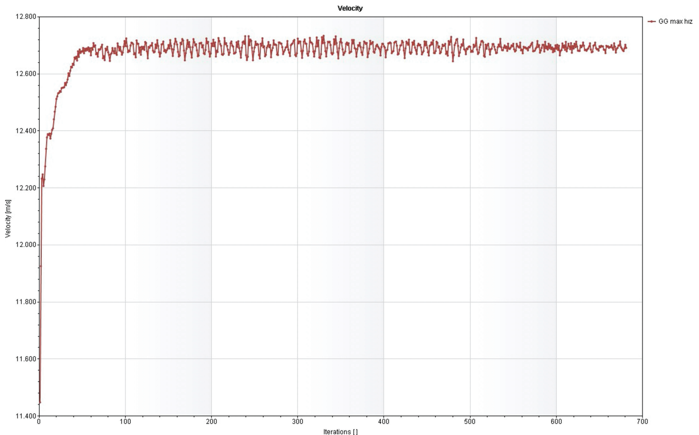
FIGURE 2. Convergence history of maximum flow velocity. The graph demonstrates the iteration history for the maximum velocity during the simulation. Following an initial steep increase, the maximum velocity oscillates within a stable, narrow band starting from approximately the 50th iteration. This stabilization confirms that numerical convergence was successfully achieved over the total 681 iterations.
